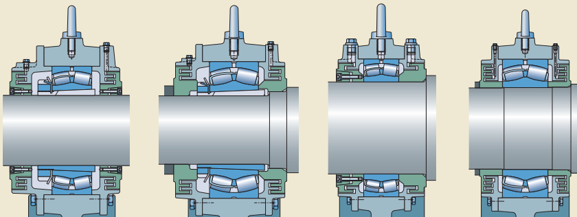
Plain shaft with bearing on an adapter sleeve
