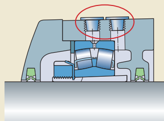
Relubrication holes
